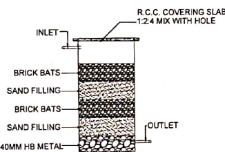
WASTE WATER RECYCLED UNIT
