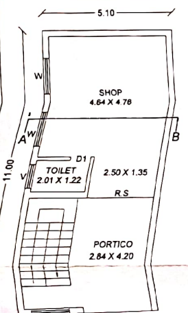
PROPOSED GROUND FLOOR PLAN (COMMERCIAL)
