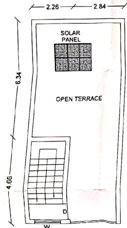
PROPOSED TERRACE FLOOR PLAN (RESIDENTIAL)
