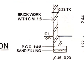
SECTION OF COMPOUND WALL
