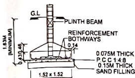
COLUMN FOOTING DETAILS
