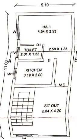
PROPOSED FIRST FLOOR PLAN (RESIDENTIAL)
