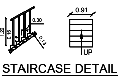
STAIRCASE DETAIL
