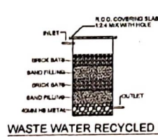
WASTE WATER RECYCLED UNIT
