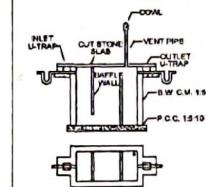
SEPTIC TANK DETAILS SIZE: 2.44X1.22X2.44
