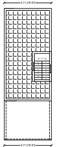
PRO.TERRACE FLOOR
