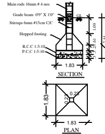
COLUMN DETAILS
