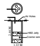
RAIN WATER HARVESTING TANK DETAIL
