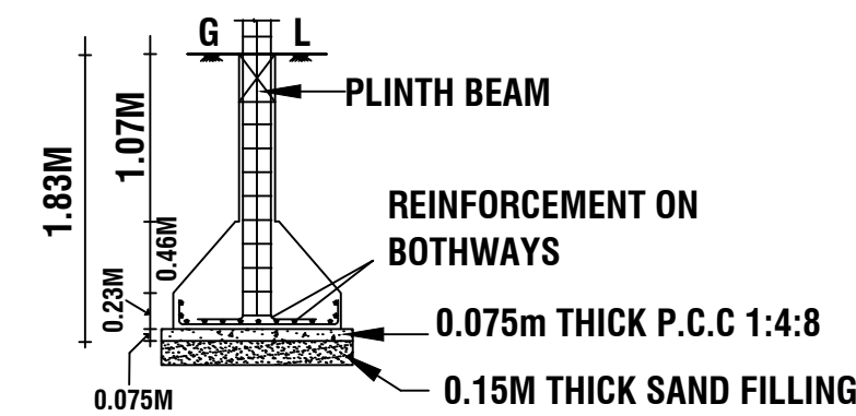
TYP. COLUMN FOOTING DETAIL
