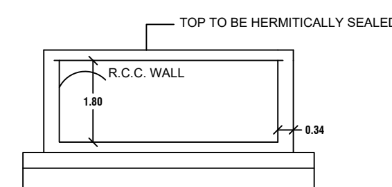
RWH SECTION (SAMPLE) RWH CAPACITY L=5000LTRS
