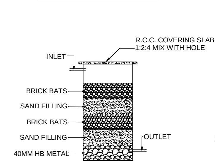
WASTE WATER RECYCLED UNIT
