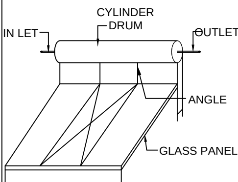
SOLAR ENERGY
