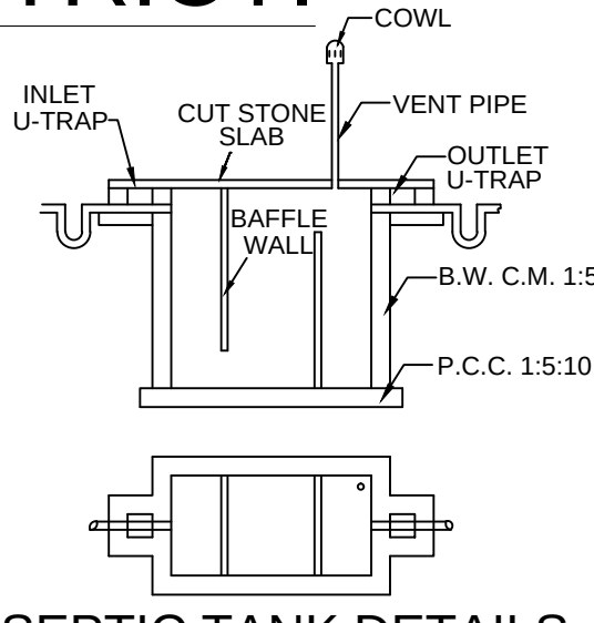
SEPTIC TANK DETAILS SIZE:2.44X1.22X2.44
