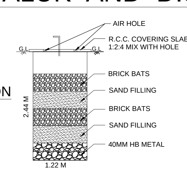
RAINWATER HARVESTING
