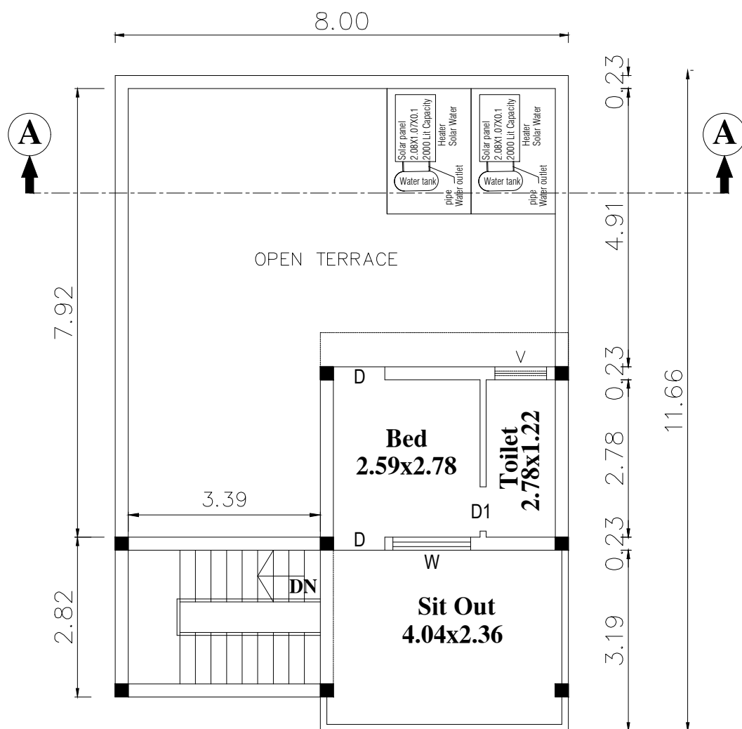
PROPOSED FIRST FLOOR AND TERRACE FLOOR PLAN
