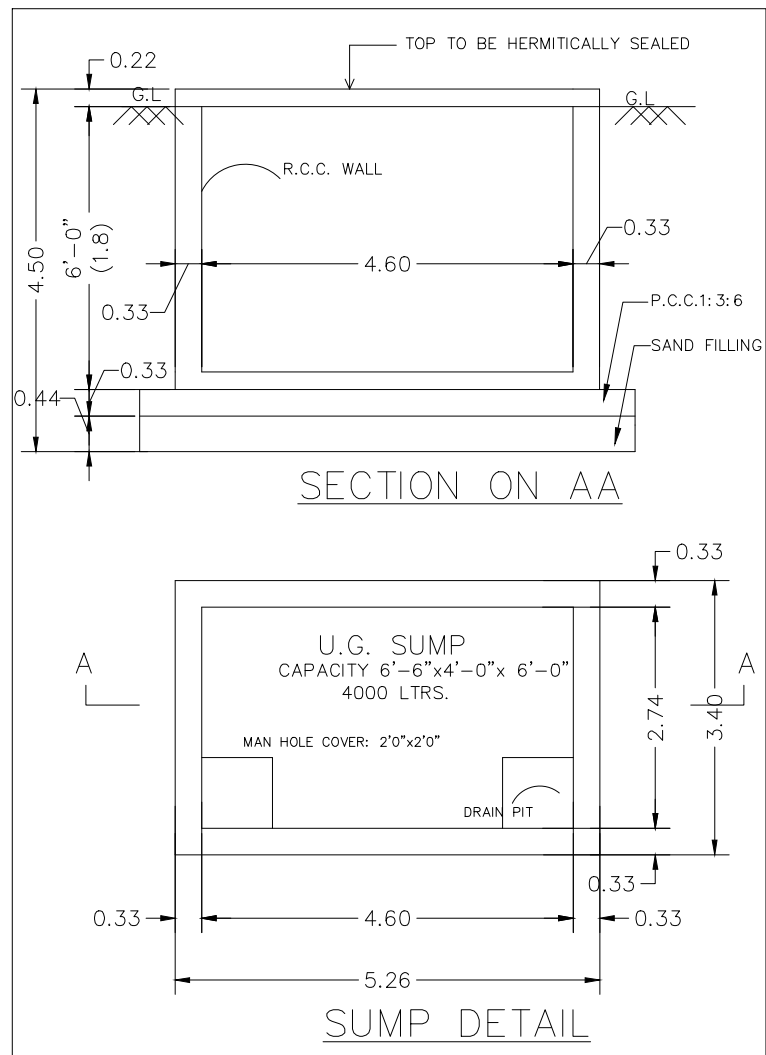
SUMP DETAIL
