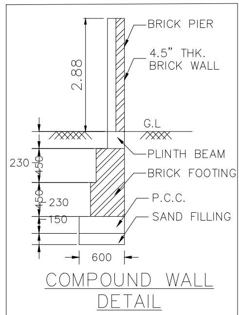
DETAIL
