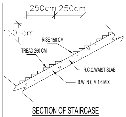
SECTION OF STAIRCASE
