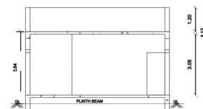
SECTION ON "X-X"
