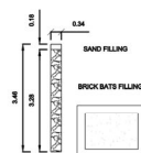
DETAILS OF PERCOLATION PIT
