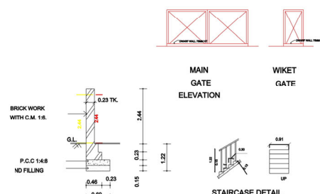
STAIRCASE DETAIL
