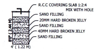
RAIN WATER HARVEST UNIT
