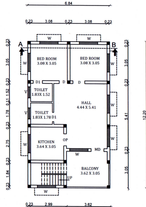
TYPICAL PRO. FIRST, SECOND, THIRD & FOURTH FLOOR PLAN
