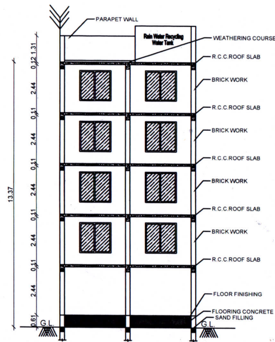
SECTION "A-B"
