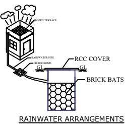
RAINWATER ARRANGEMENTS
