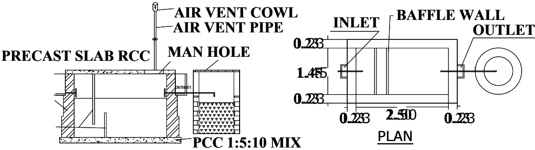
SECTION SEPTIC TANK DETAILS
