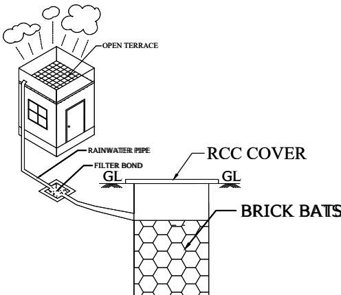
RAINWATER ARRANGEMENTS
