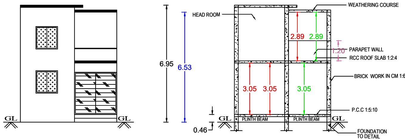
FRONT ELEVATION.
