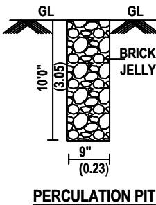
PERCOLATION PIT
