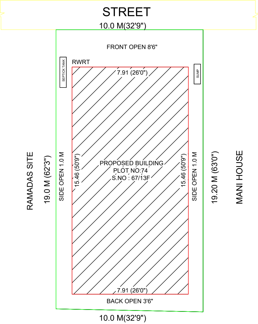
GOVINDHASWAMY SITE SITE PLAN
