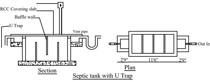
Septic tank with U Trap
