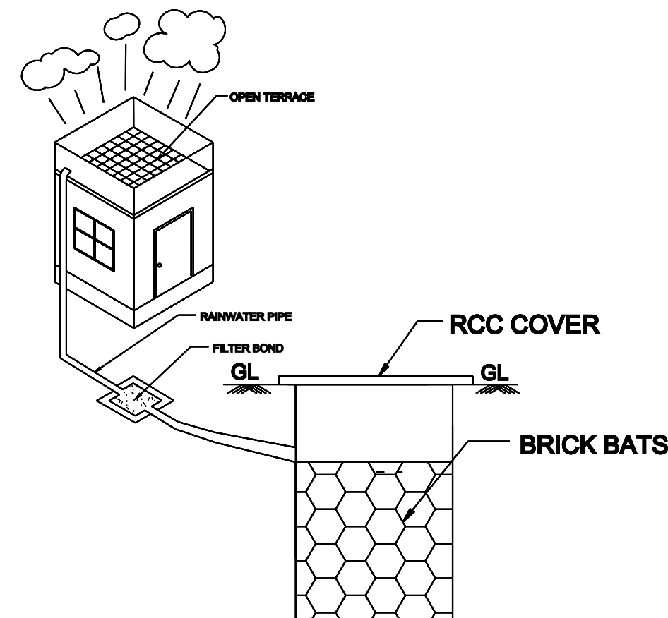
RAINWATER ARRANGEMENTS
