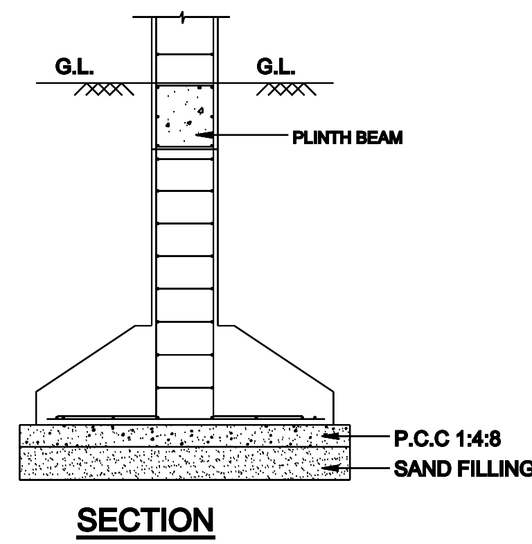
SECTION
