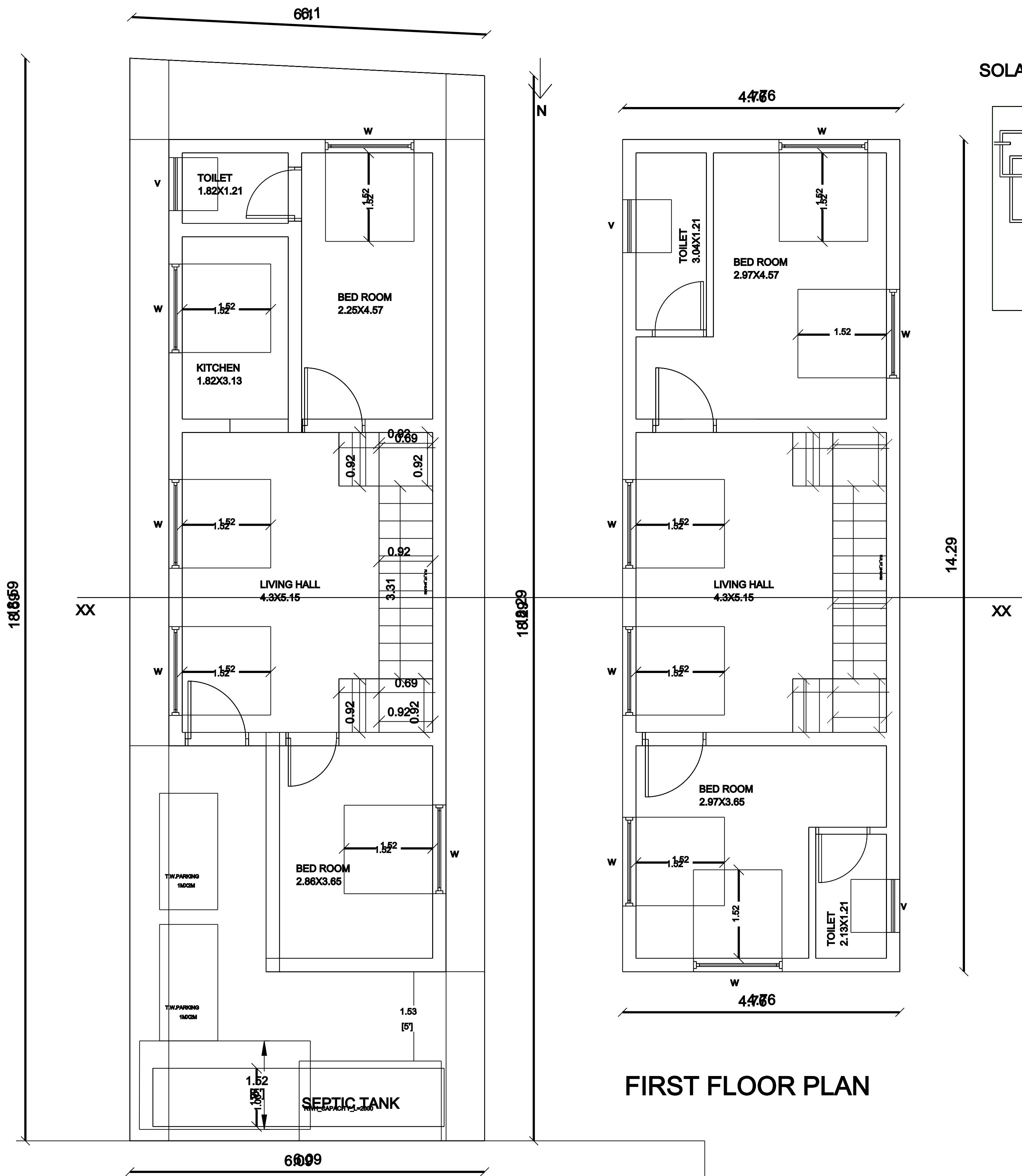
PRO. GROUND FLOOR PLAN ROAD WIDTH 6.7 M
