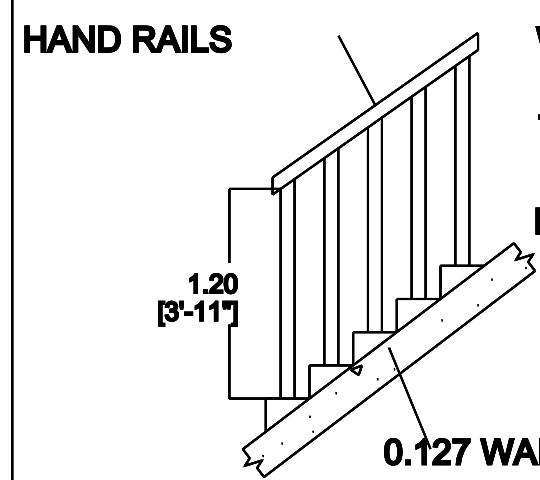
STAIRCASE DETAILS
