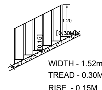
STAIRCASE DETAILS
