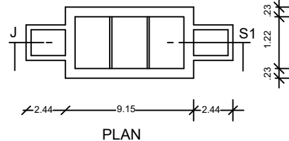
SEPTIC TANK DETAILS
