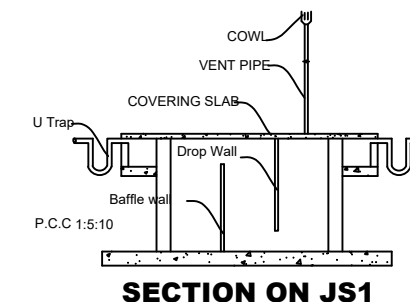
SECTION ON 'JS1'
