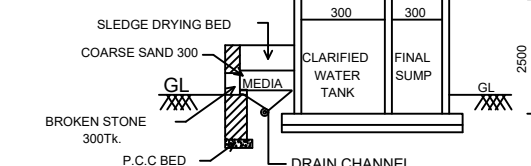
SECTION ON 'BB'
