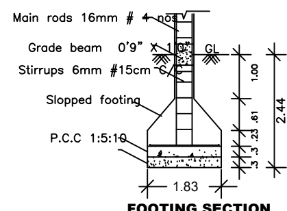
FOOTING SECTION
