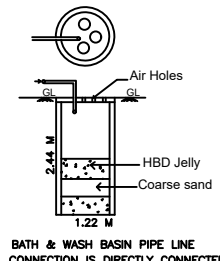
WASTE WATER RECYCLING TANK DETAIL
