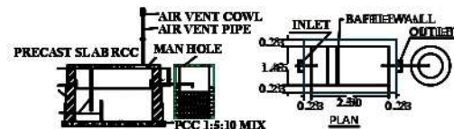
SECTION SEPTIC TANK DETAILS
