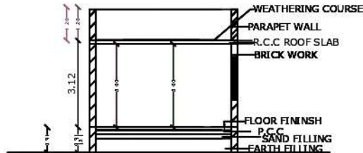
SECTION XX
