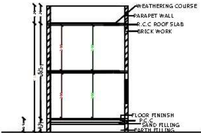
SECTION XX
