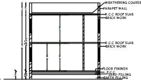
SECTION XX
