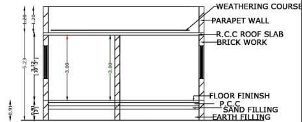
SECTION XX
