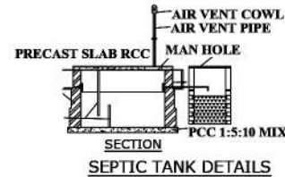
SECTION SEPTIC TANK DETAILS
