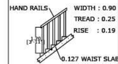
STAIRCASE DETAILS
