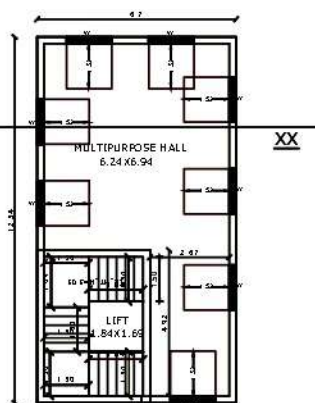
PRO. SECOND FLOOR
