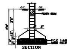
SECTION
