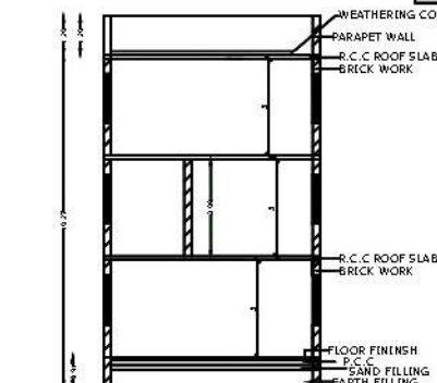
SECTION XX
