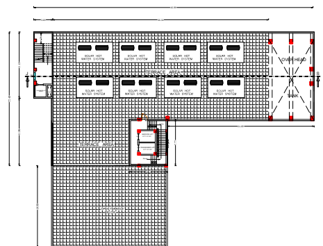
OPEN TERRACE FLOOR PLAN
