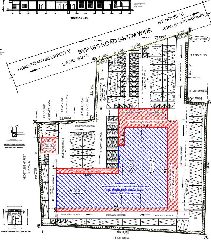
SITE PLAN
