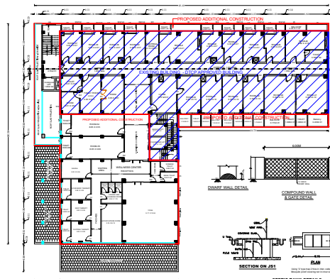
EXG. & PRO. ADDITIONAL THIRD FLOOR PLAN
