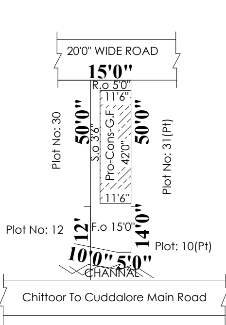
SITE PLAN
