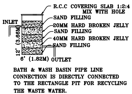
Section - Septic tank & Soak pit
