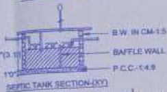
SEPTIC TANK SECTION (XY)
