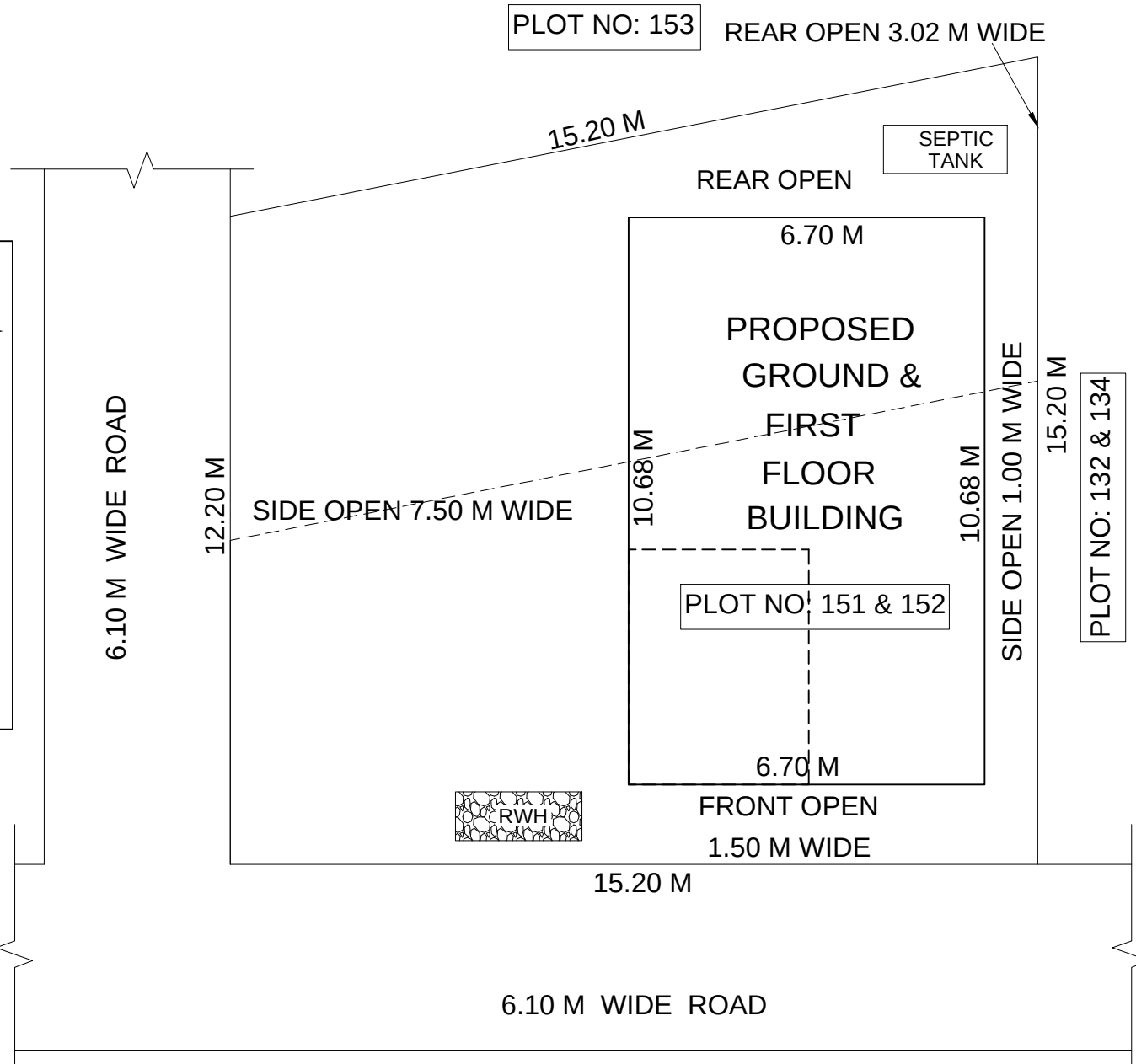
SITE PLAN
