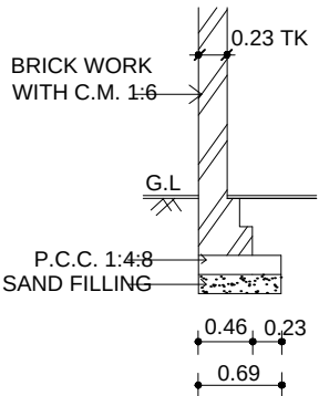
SECTION OF COMPOUND WALL
