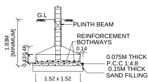
COLUMN FOOTING DETAILS
