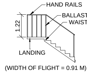
STAIRCASE DETAIL
