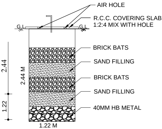
RAINWATER HARVESTING
