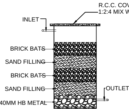
WASTE WATER RECYCLED UNIT
