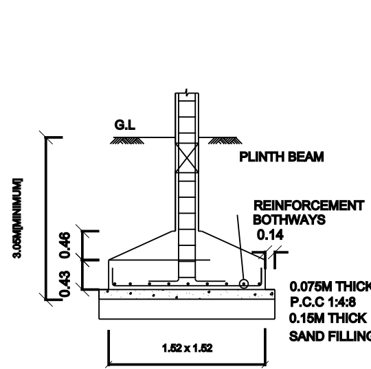
COLUMN FOOTING ( REFER STRUCTURAL DRAWING )
