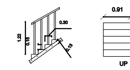
STAIRCASE DETAIL
