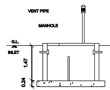
SECTION OF SEP.TANK
