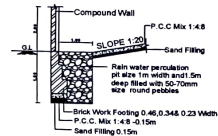
RAINWATER HARVESTING TRENCH
