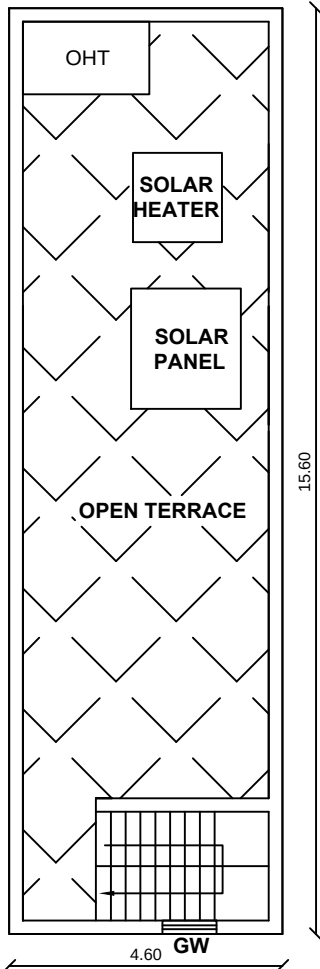
TERRACE FLOOR PLAN
