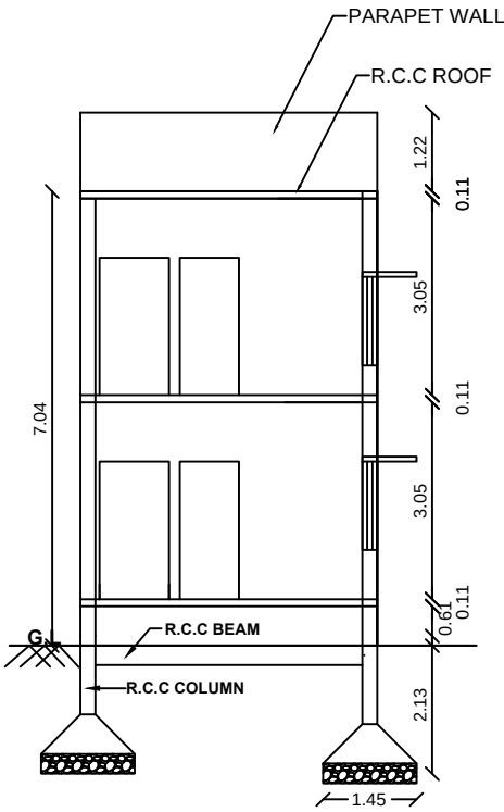
SECTION ON A.A
