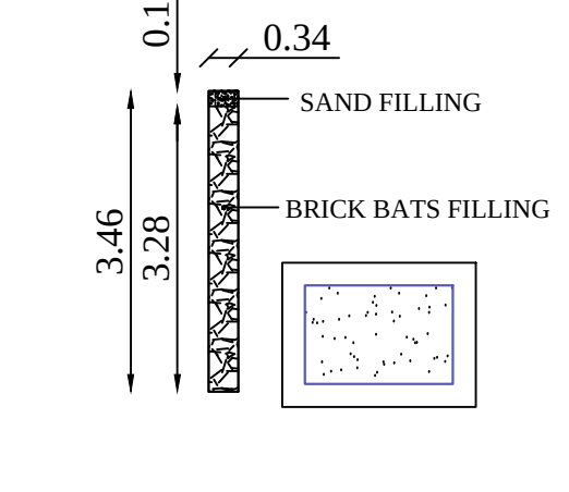
DETAILS OF PERCOLATION PIT
