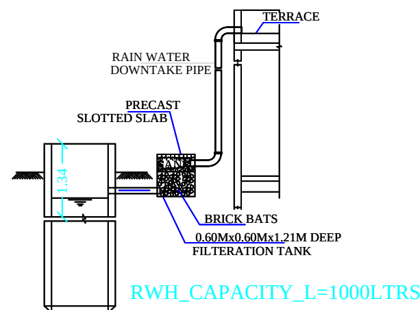
RAIN WATER HARVESTING SYSTEM
