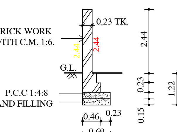
SECTION OF COMPOUND WALL
