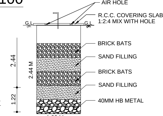
RAINWATER HARVESTING SECTION OF COMPOUND WALL
