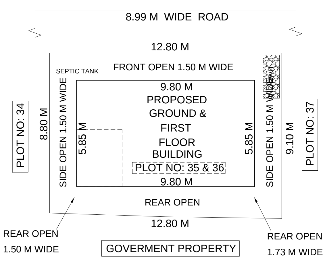
SITE PLAN
