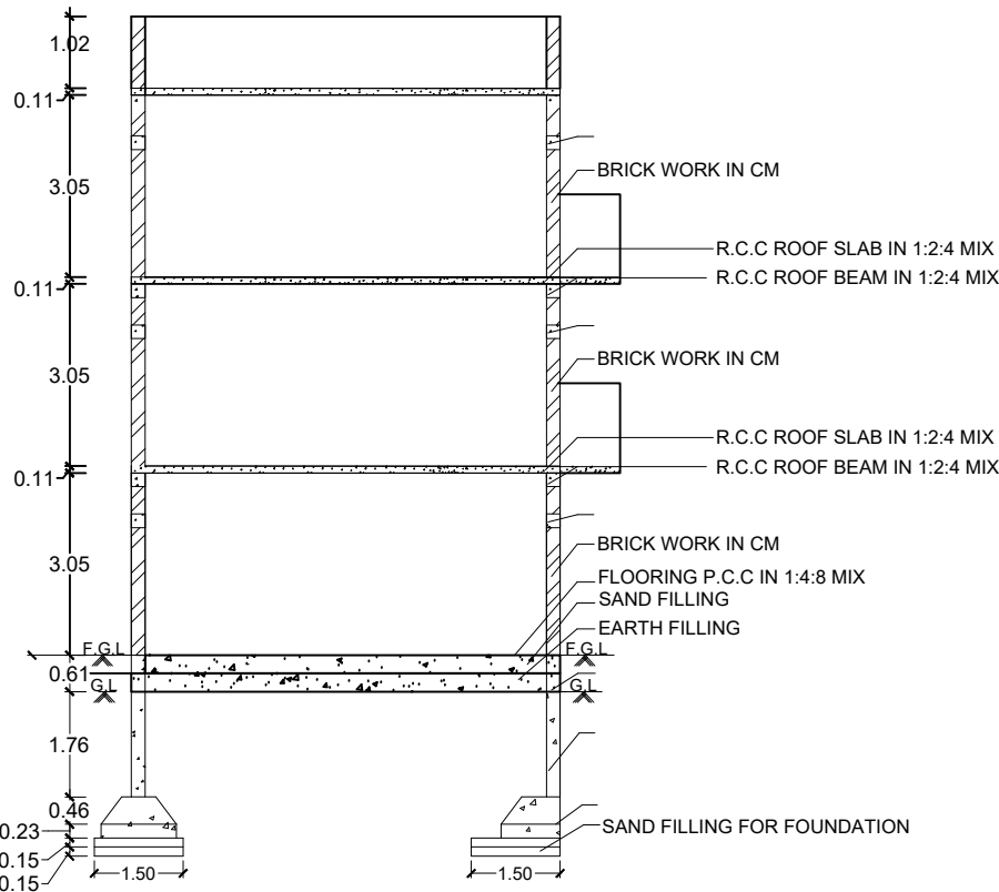
SECTION ON-AA
