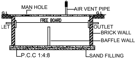
SECTION 'Y-Y' SEPTIC TANK DETAILS
