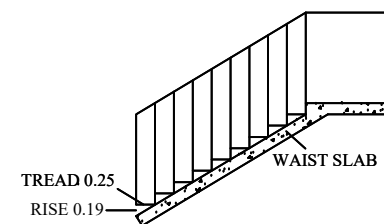
STAIRCASE DETAILS: RISE : 0.19m TREAD : 0.25m WIDTH : 1.0m HEIGHT : 1.25 m
