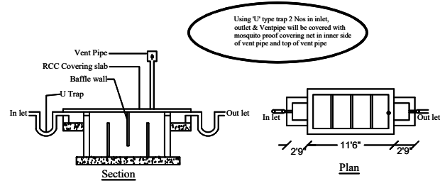
SEPTIC TANK WITH U TRAP
