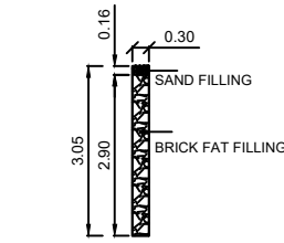
DETAILS OF PERCOLATION PIT
