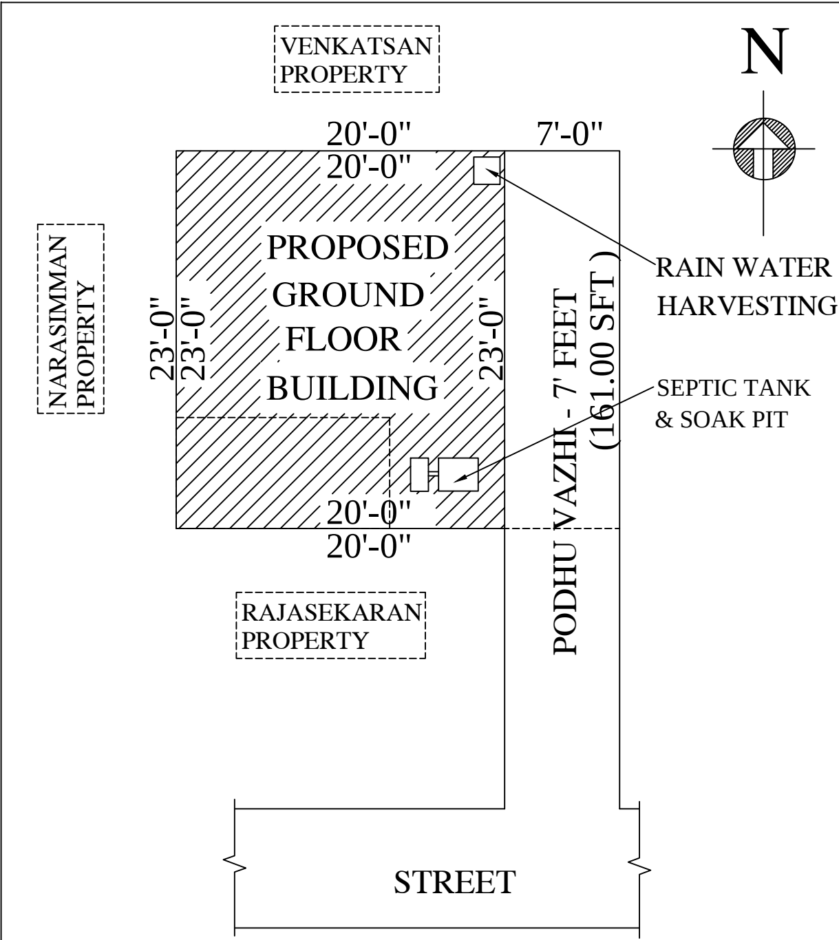
SITE PLAN
