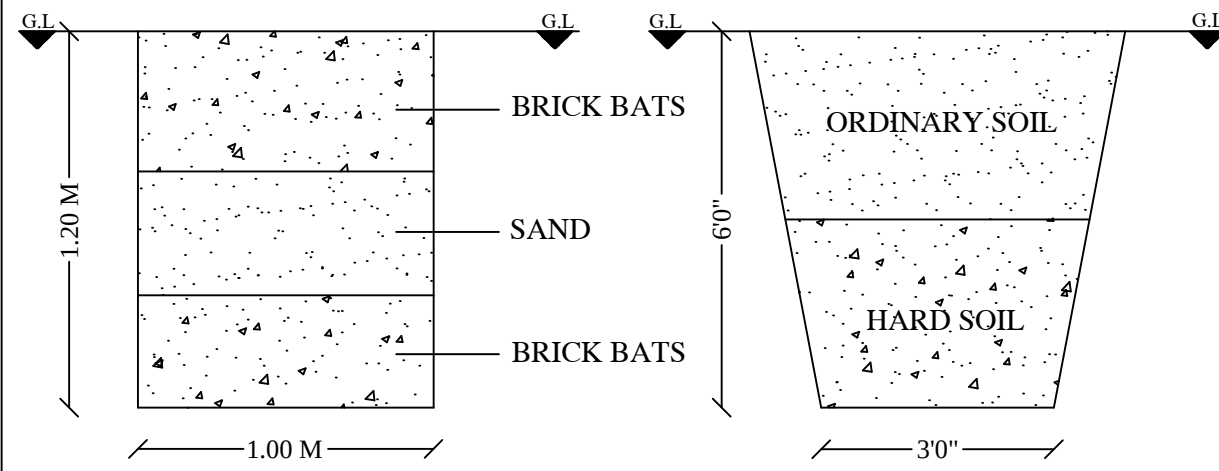
RAINWATER HARVESTING
