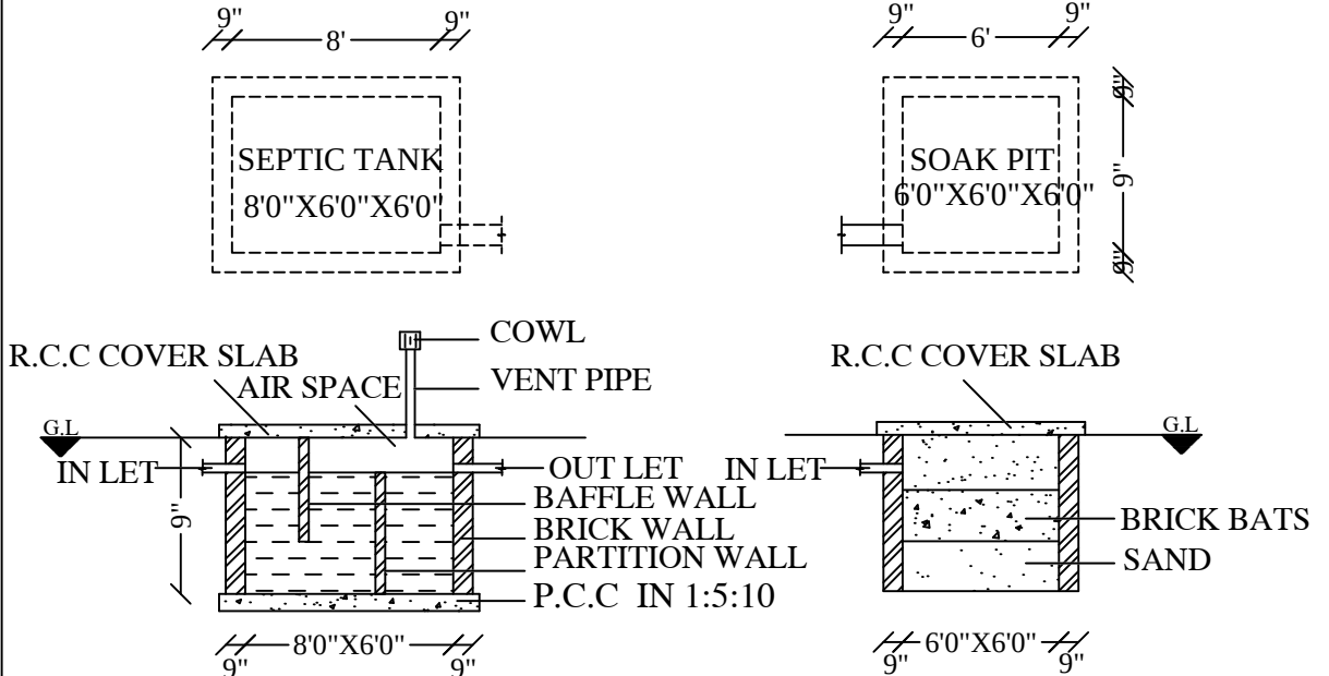
SEPTIC TANK AND SOAKPIT DETAILS
