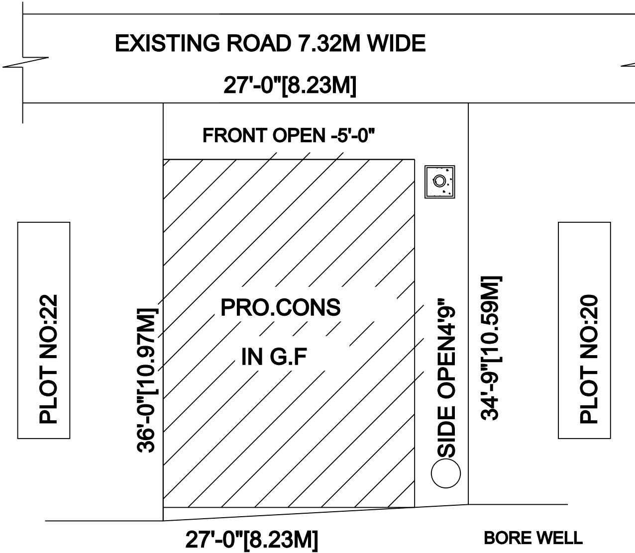
SITE PLAN
