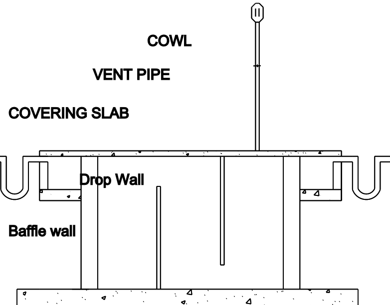
SECTION ON JS1
