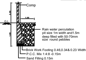
RAINWATER HARVESTING TRENCH
