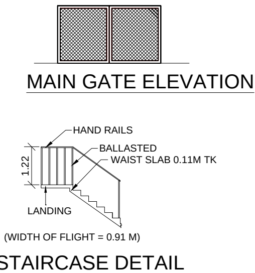
STAIRCASE DETAIL
