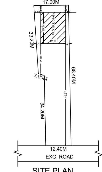
SITE PLAN (SCALE 1:800)
