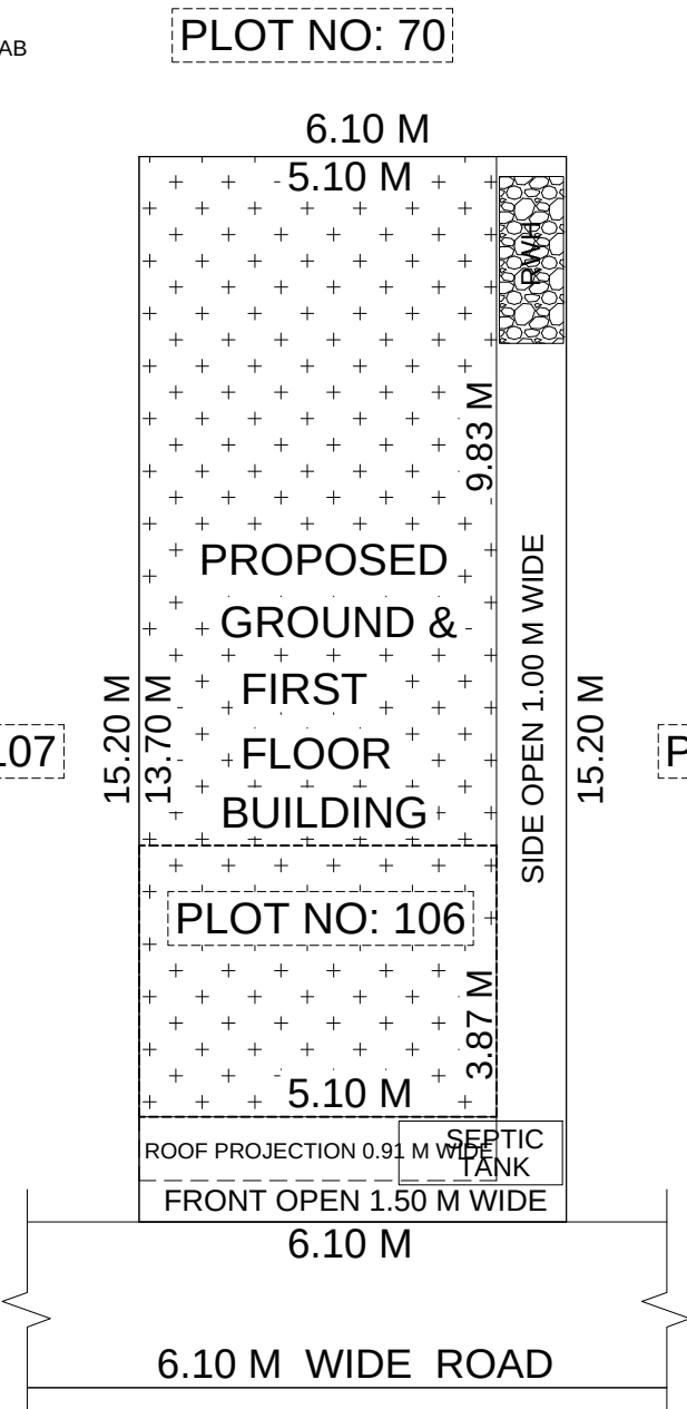
SITE PLAN
