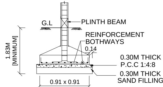
COLUMN FOOTING DETAILS
