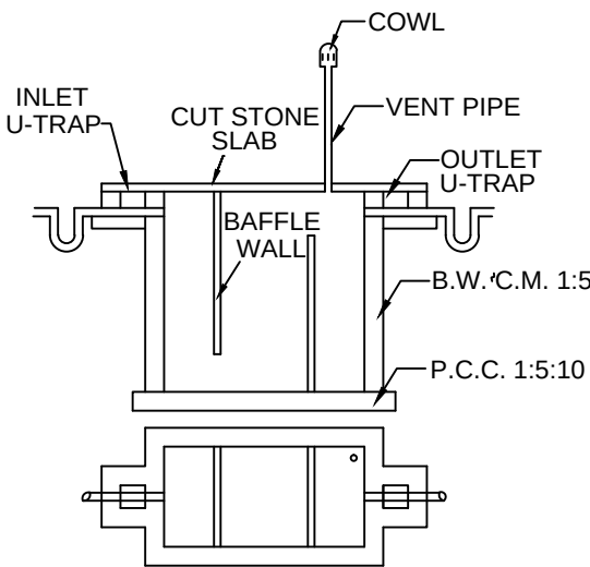
SEPTIC TANK DETAILS SIZE:2.44X1.22X2.44
