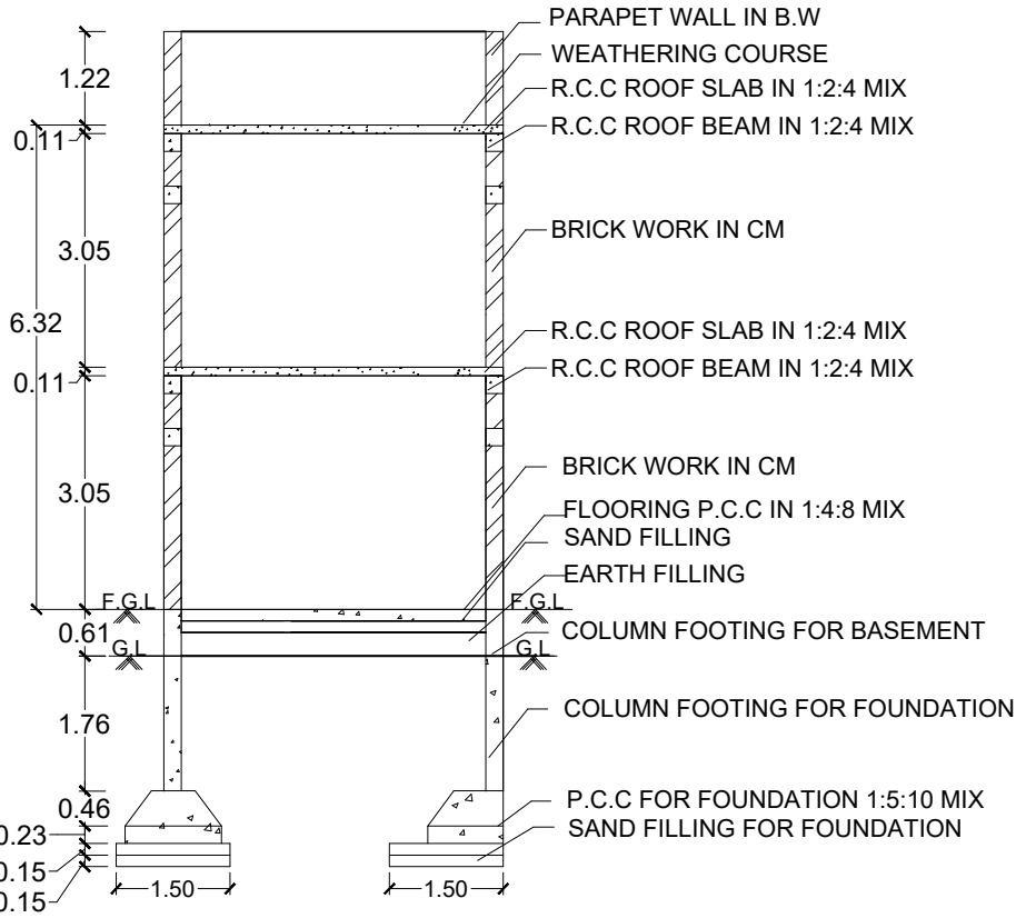
SECTION ON-AA
