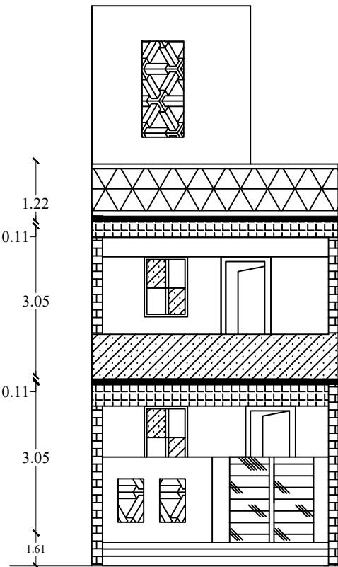
FRONT ELEVATION
