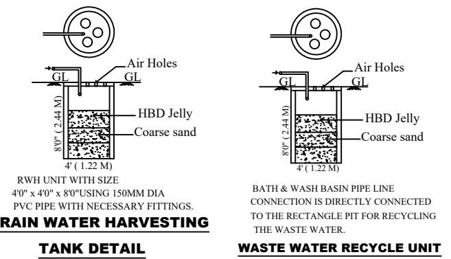
TANK DETAIL
