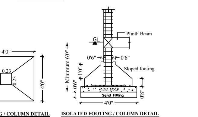
FOOTING / COLUMN DETAIL
