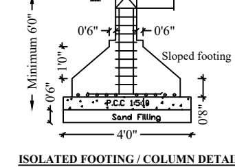
ISOLATED FOOTING / COLUMN DETAIL
