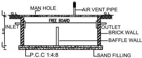
SECTION 'Y-Y'
