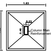
PLAN OF FOOTING
