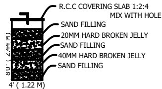
WATER HARVEST UNIT
