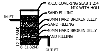
WASTE WATER RECYCLE UNIT
