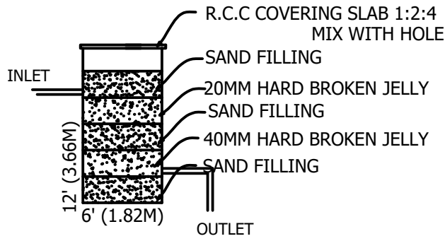
WASTE WATER RECYCLE UNIT
