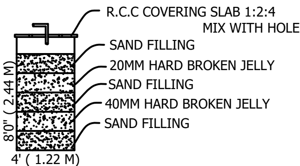
RAIN WATER HARVEST UNIT
