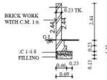
SECTION OF COMPOUND WALL
