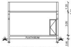
SECTION ON "X-X"
