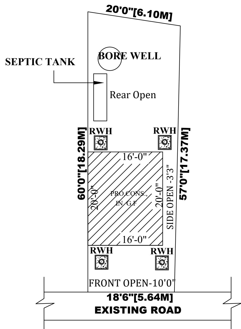
SITE PLAN
