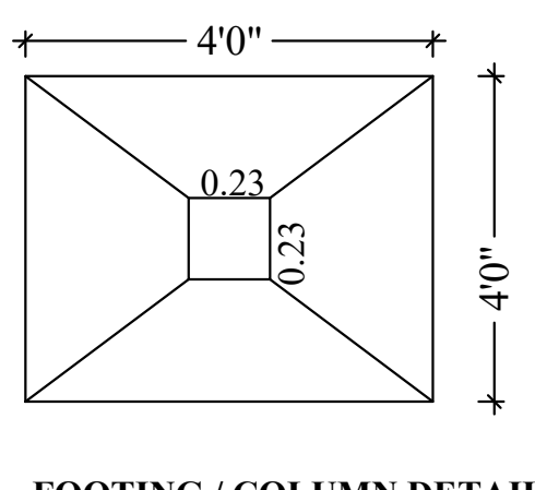
FOOTING / COLUMN DETAIL
