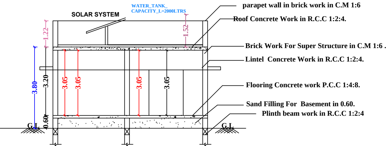
SECTION-AB
