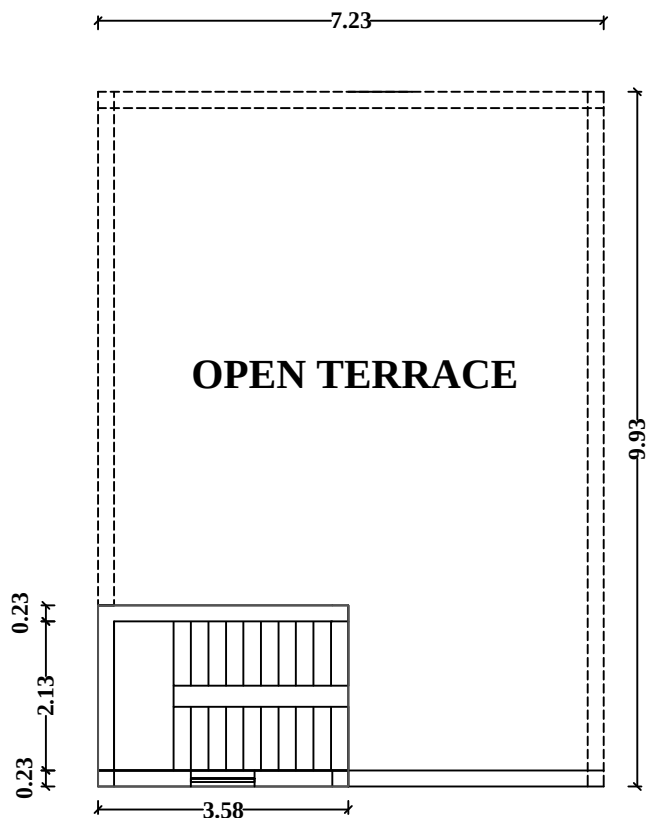
FLOOR-1 PRO.TERRACE FLOOR PLAN
