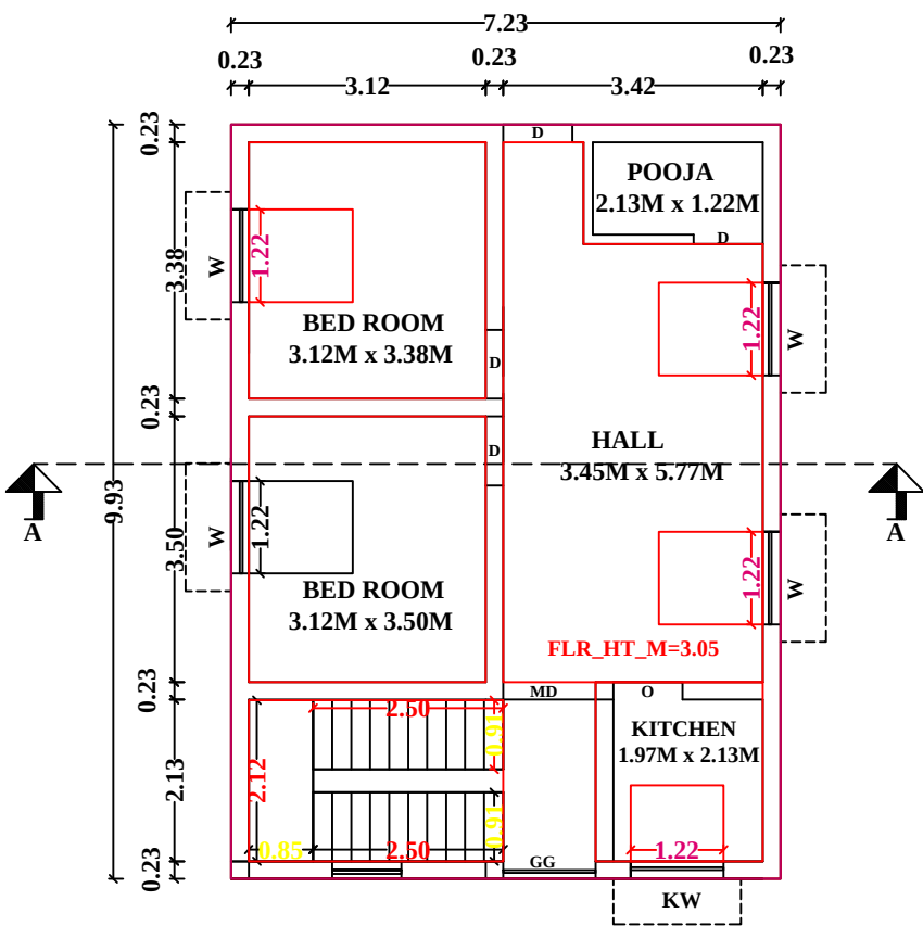
FLOOR-GROUND PRO.GROUND FLOOR PLAN
