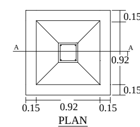
FOUNDATION DETAILS
